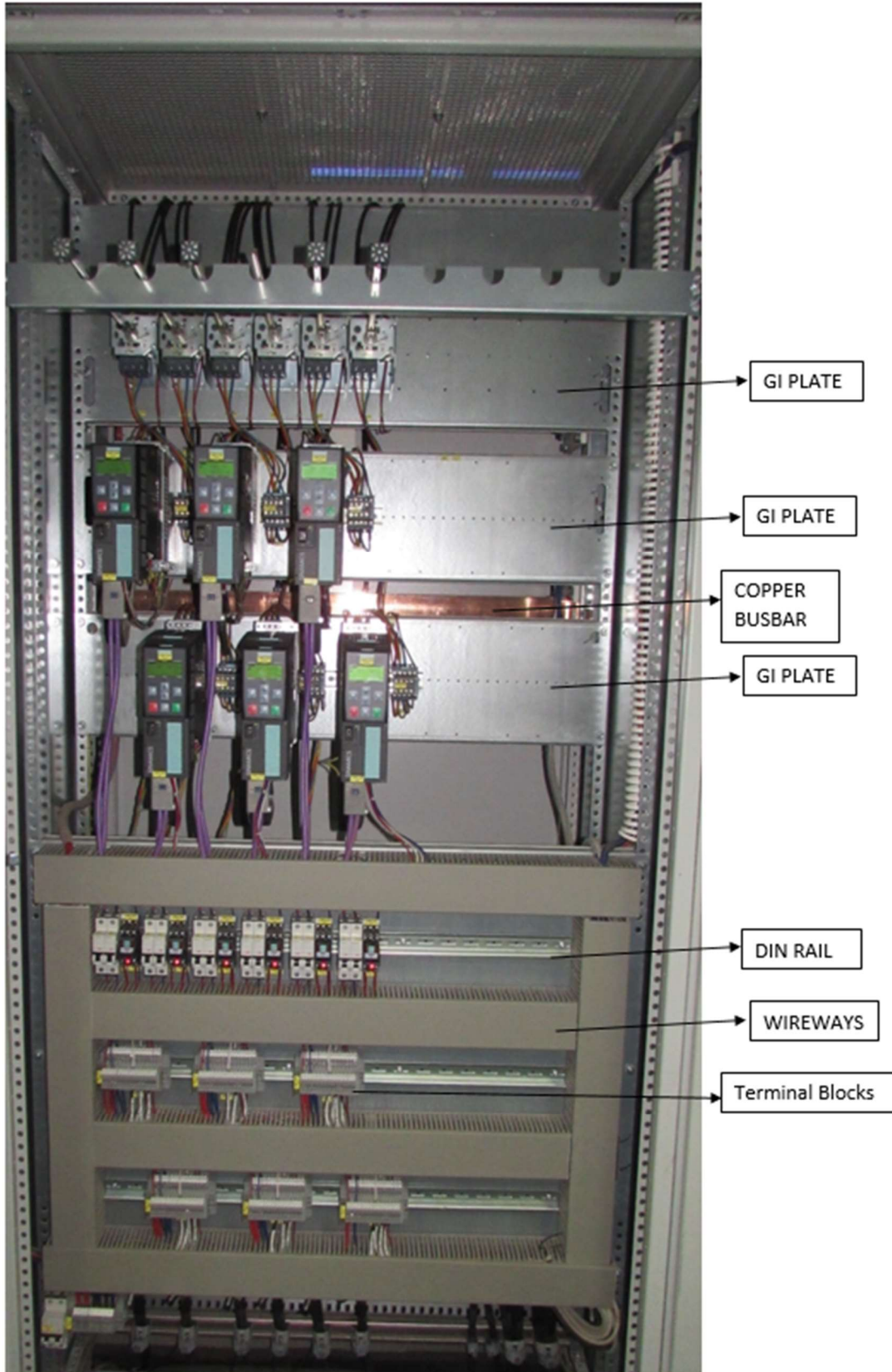
EXISTING LT DRIVE PANEL SET UP: (PICTURE-2)
